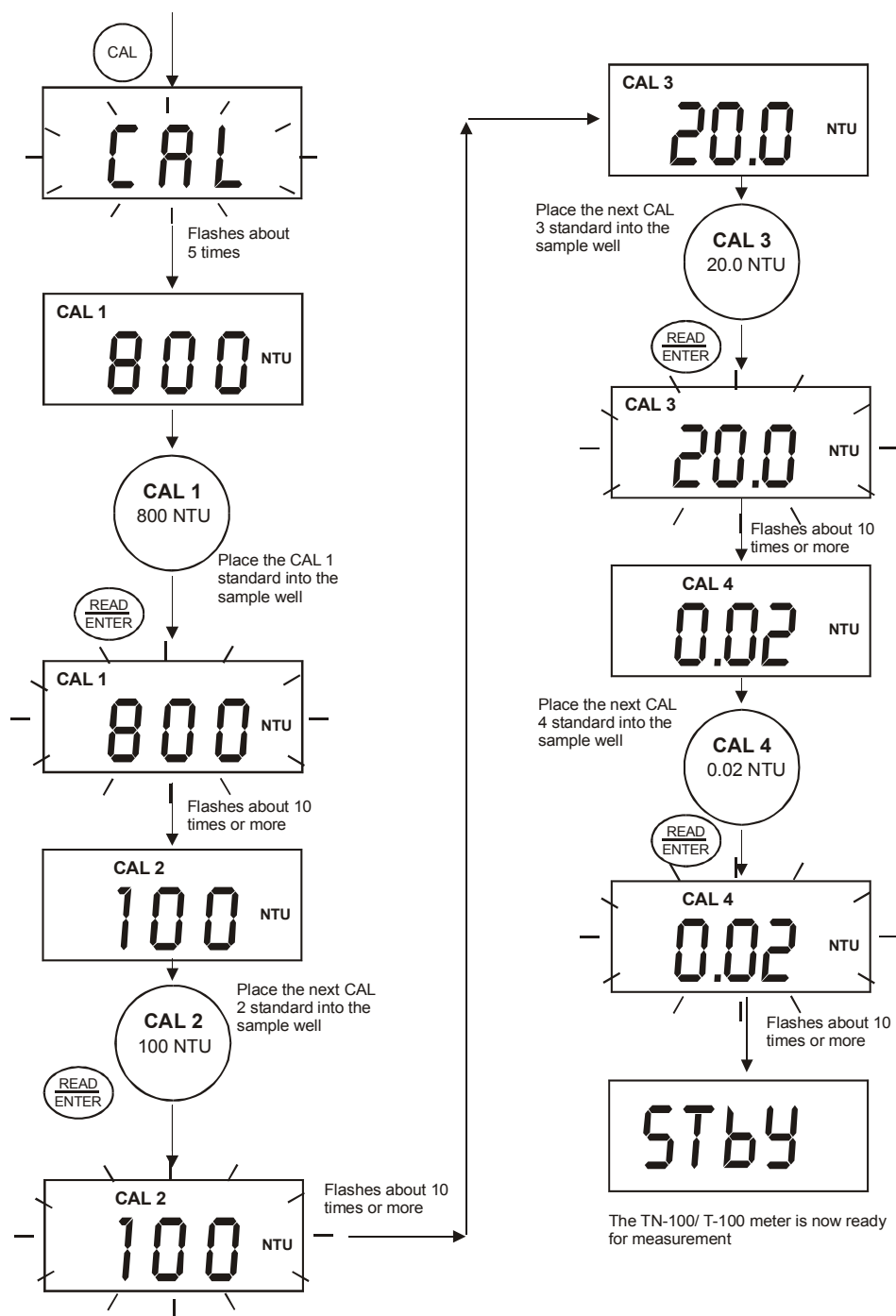
Figure 4: Calibration Sequence
