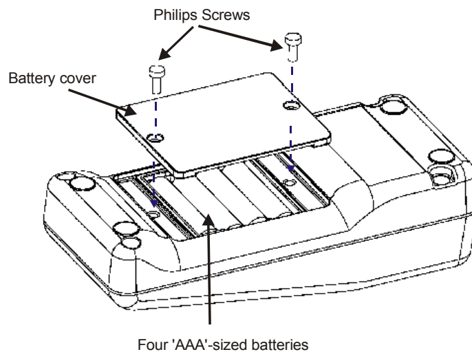
Figure 3: Battery Installation
